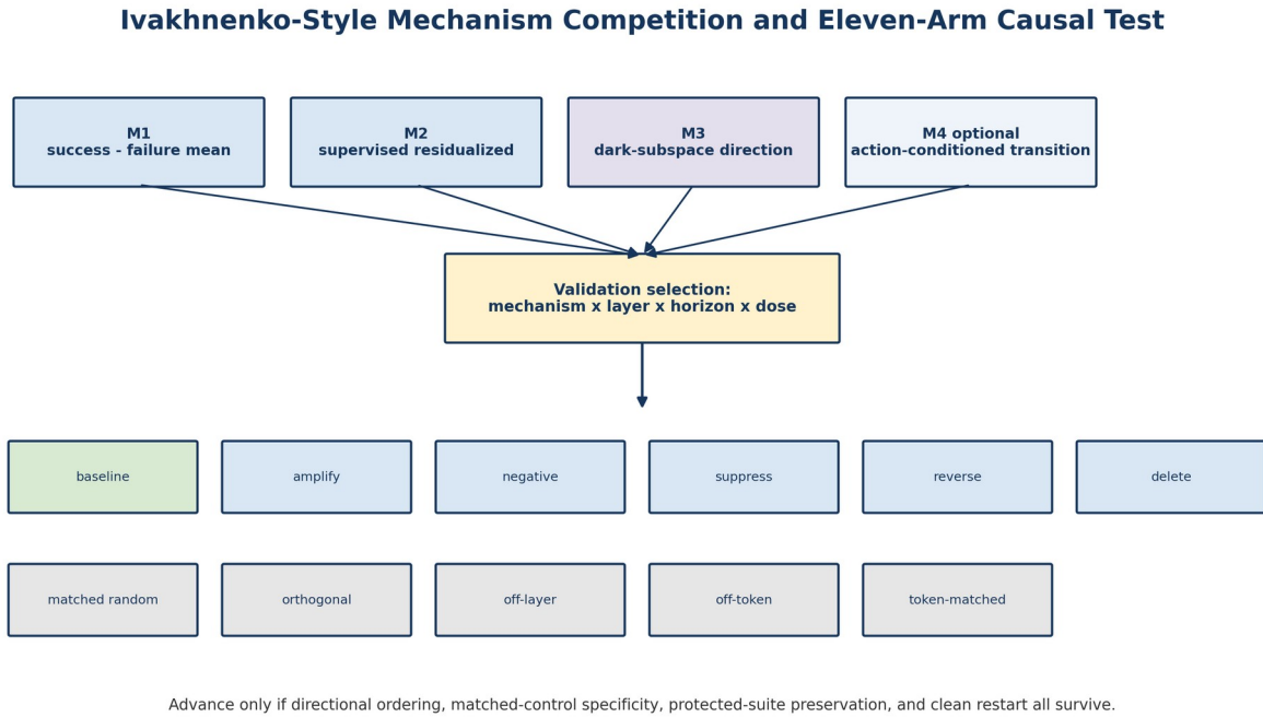
Figure 9. Competing direction mechanisms enter a validation-selected eleven-arm causal experiment.
